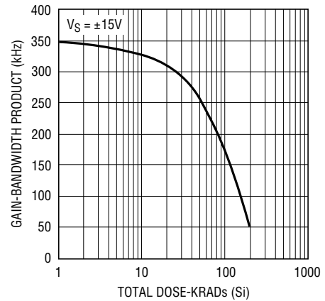
Gain-Bandwidth Product
